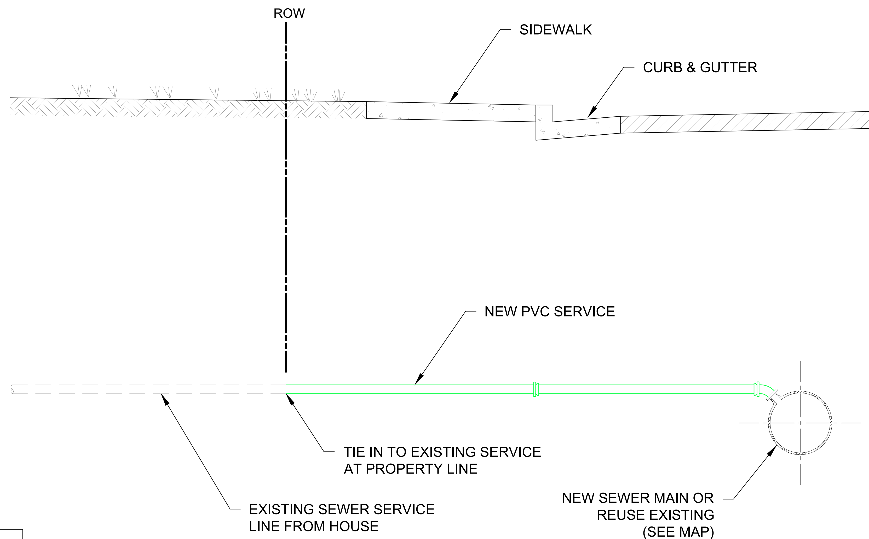
SEWER SERVICE DETAIL
