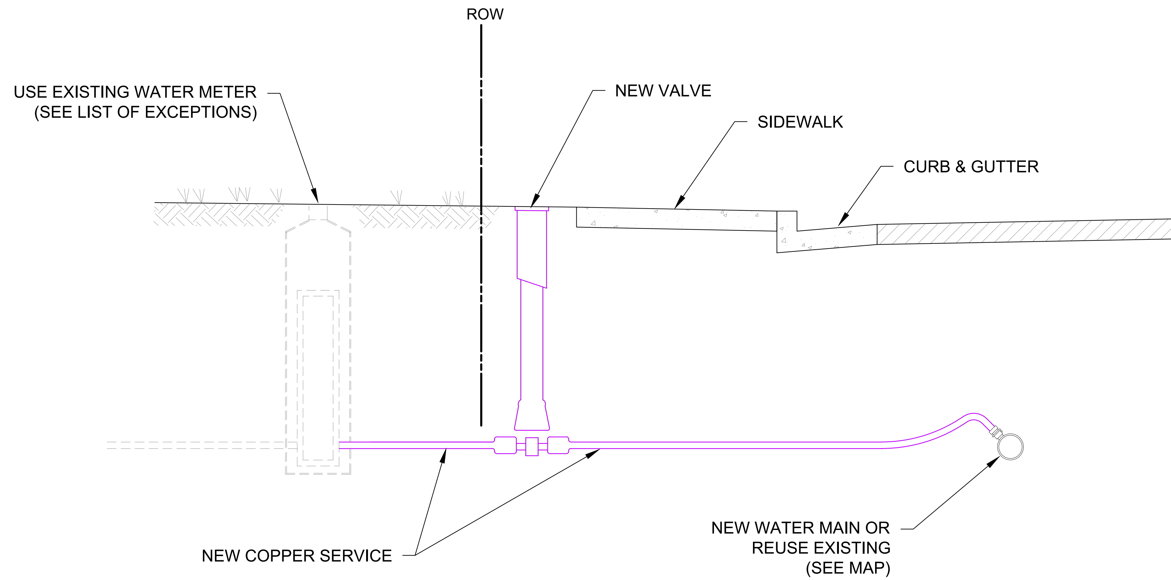
WATER SERVICE DETAIL
